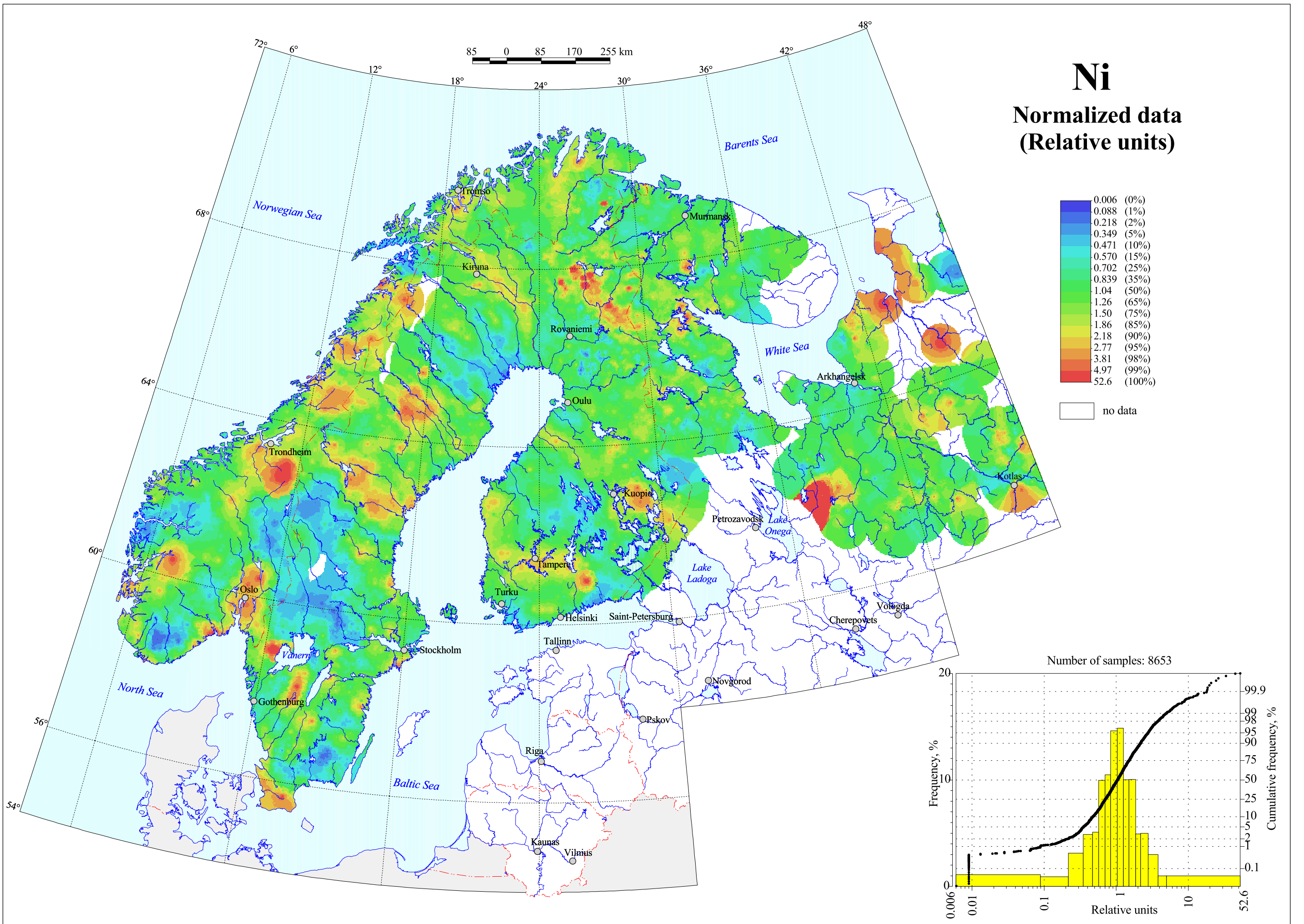
Nickel in Till, Grain Size <0.06 mm
